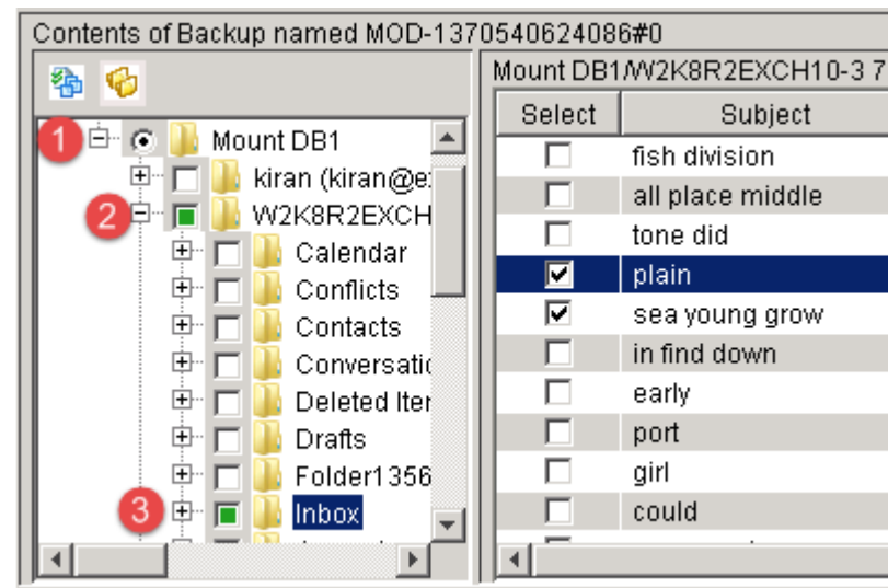
Figure 10 Database, user mailbox, and user mailbox folder levels
